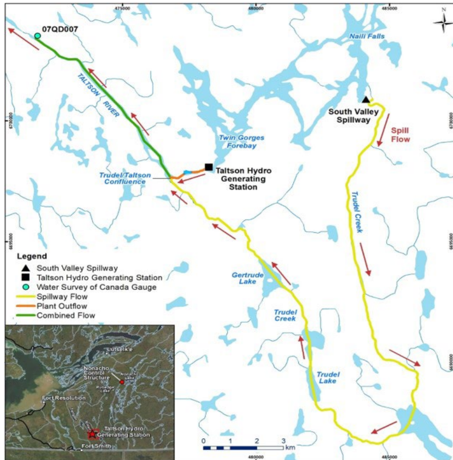
Figure 1. Taltson Hydro Facility Spillway Map
