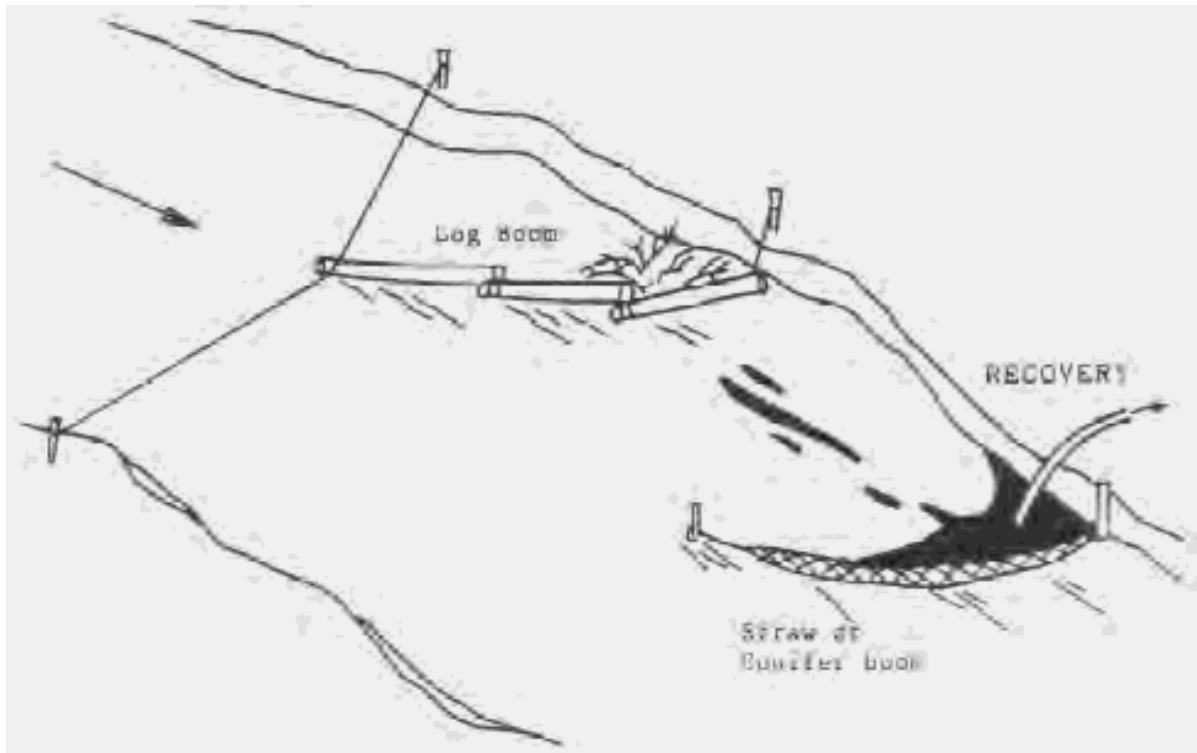
Figure E-3: Boom Usage
