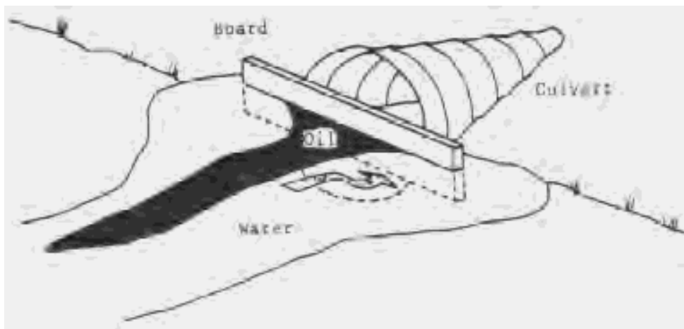
Figure E-5: Weirs
