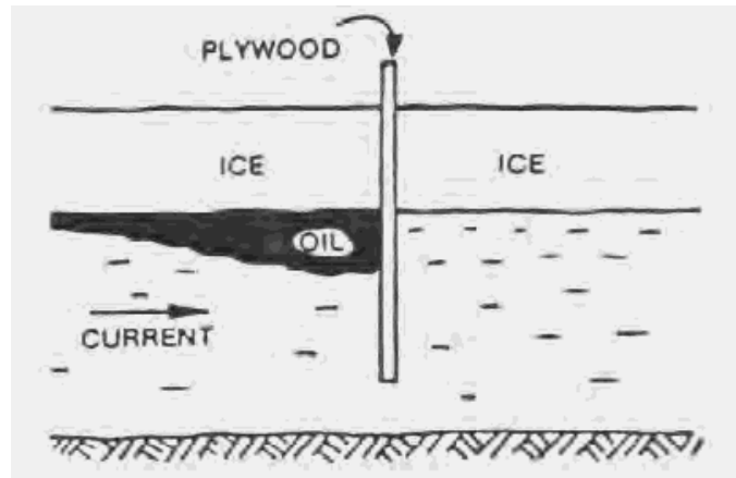
Figure E-9: Vertical Barriers
