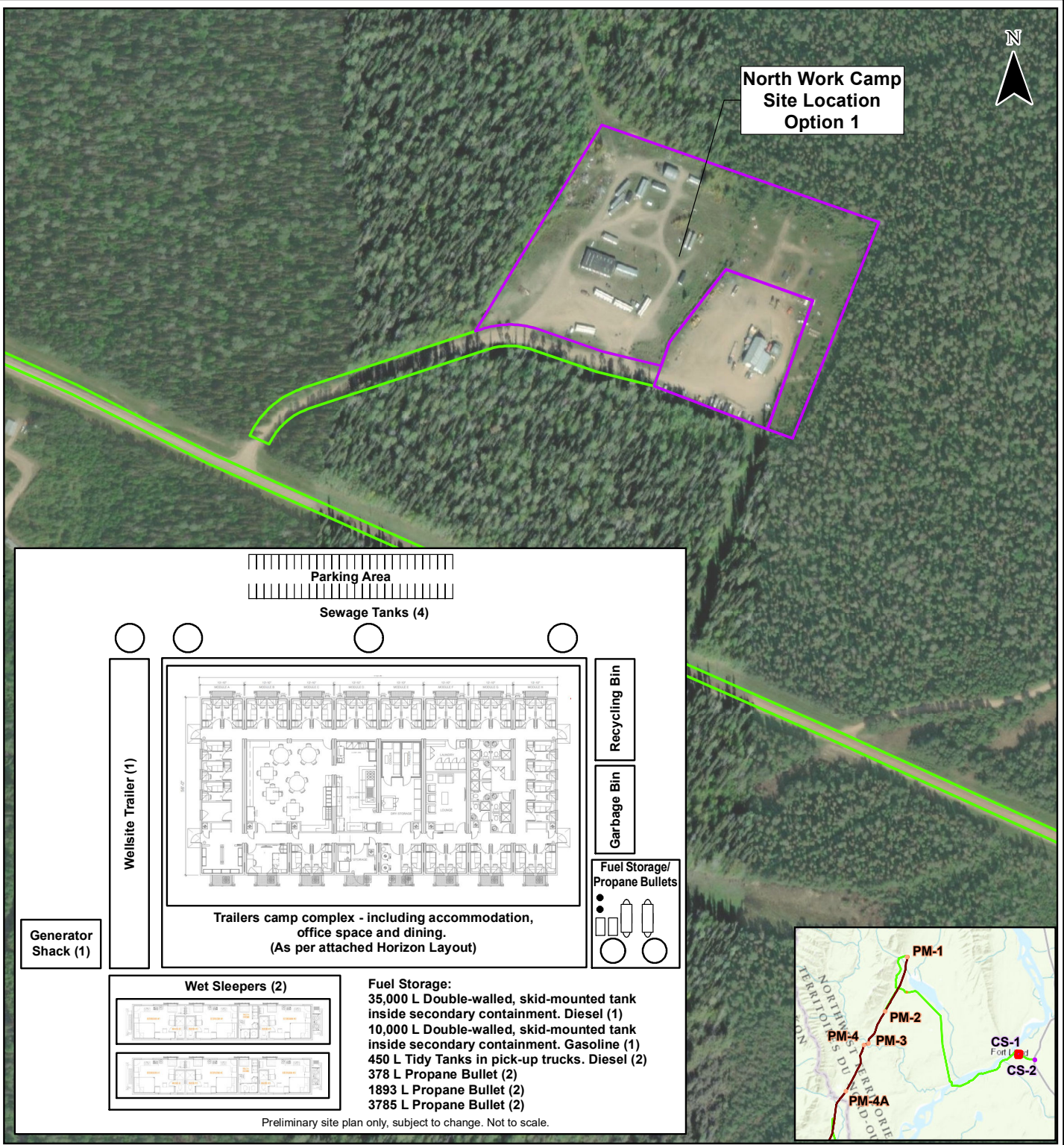
FIGURE 1-7 NORTH WORK CAMP SITE LOCATION OPTION 1
