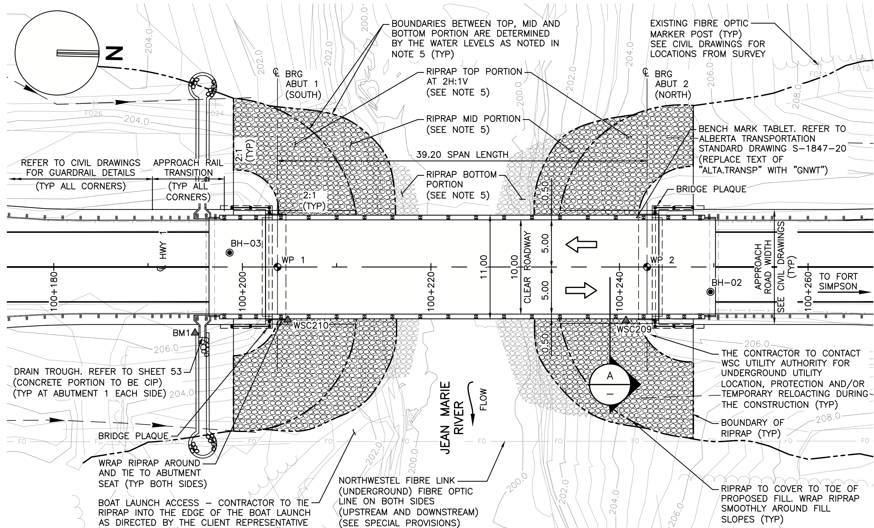
PLAN SCALE 1:250
