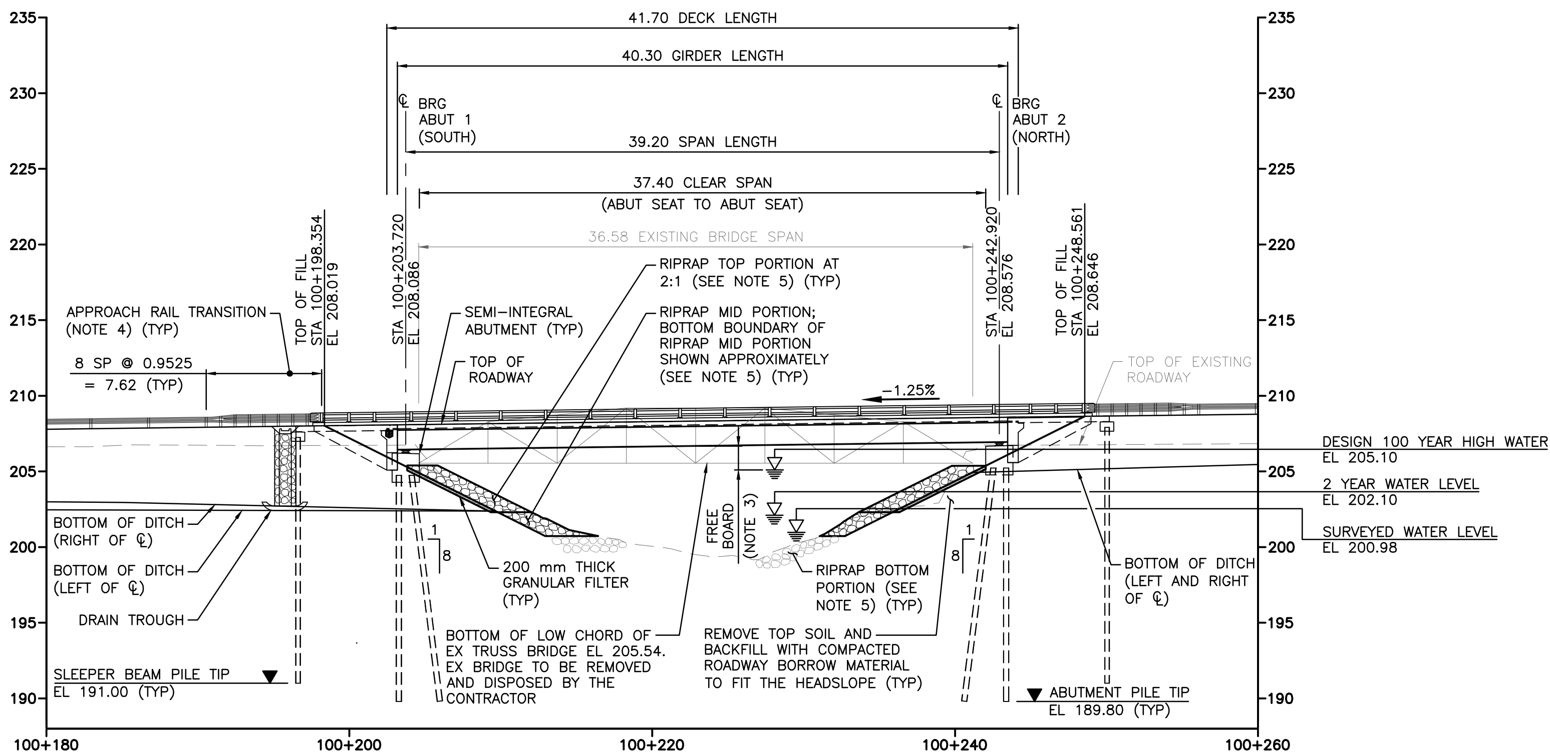
ELEVATION SCALE 1:250
